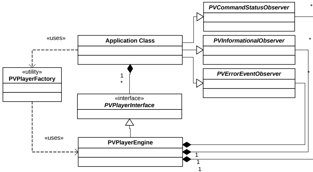
Figure 2: Class Diagram
