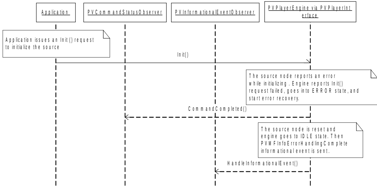
Figure 40: Error Recovery During Initialization
