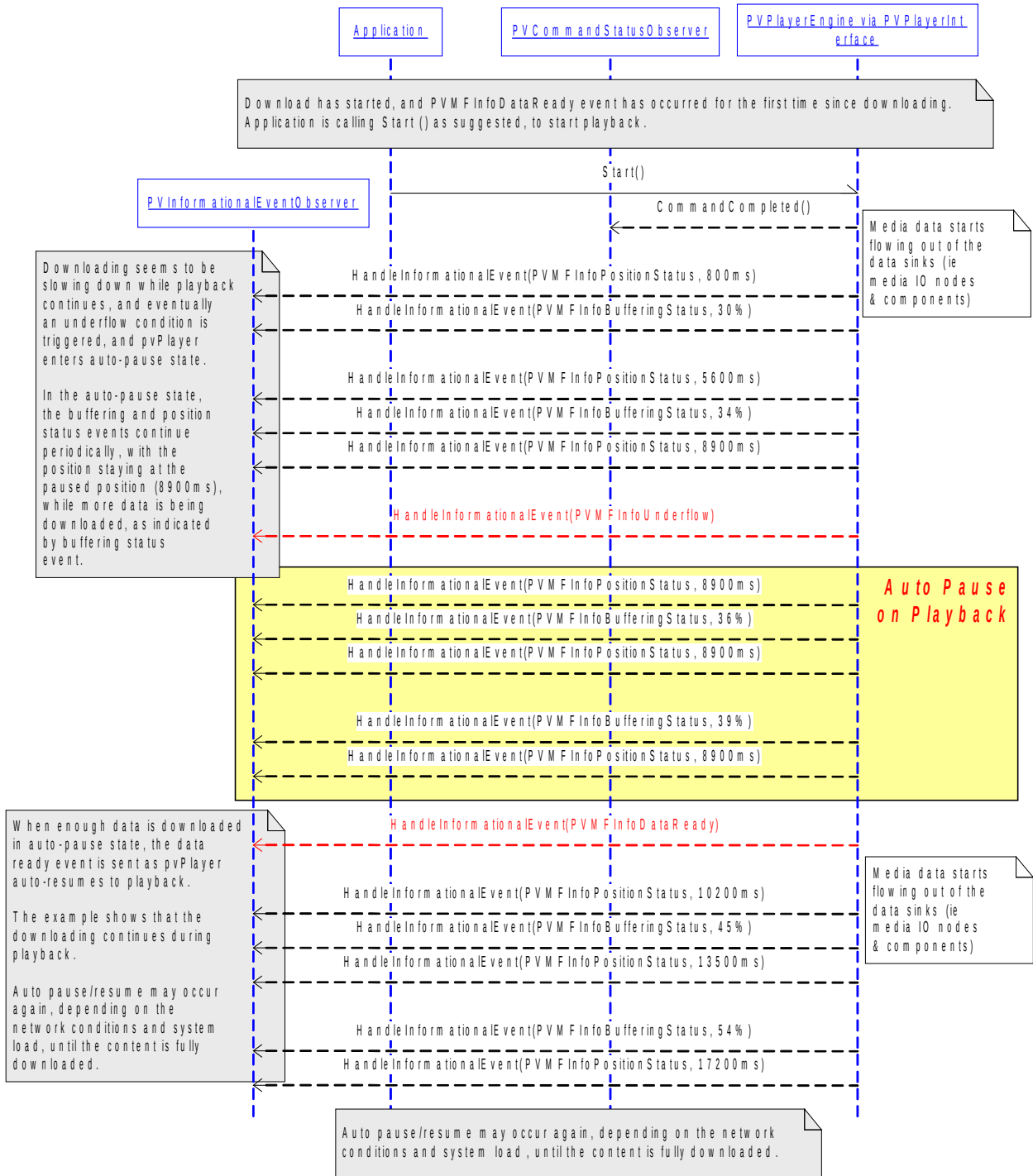
Figure 39: Auto-Pause-Resume in Progressive Download Session
