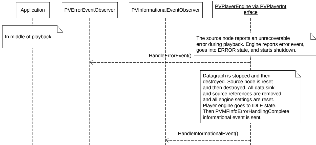
Figure 42: Unrecoverable Error Handling
