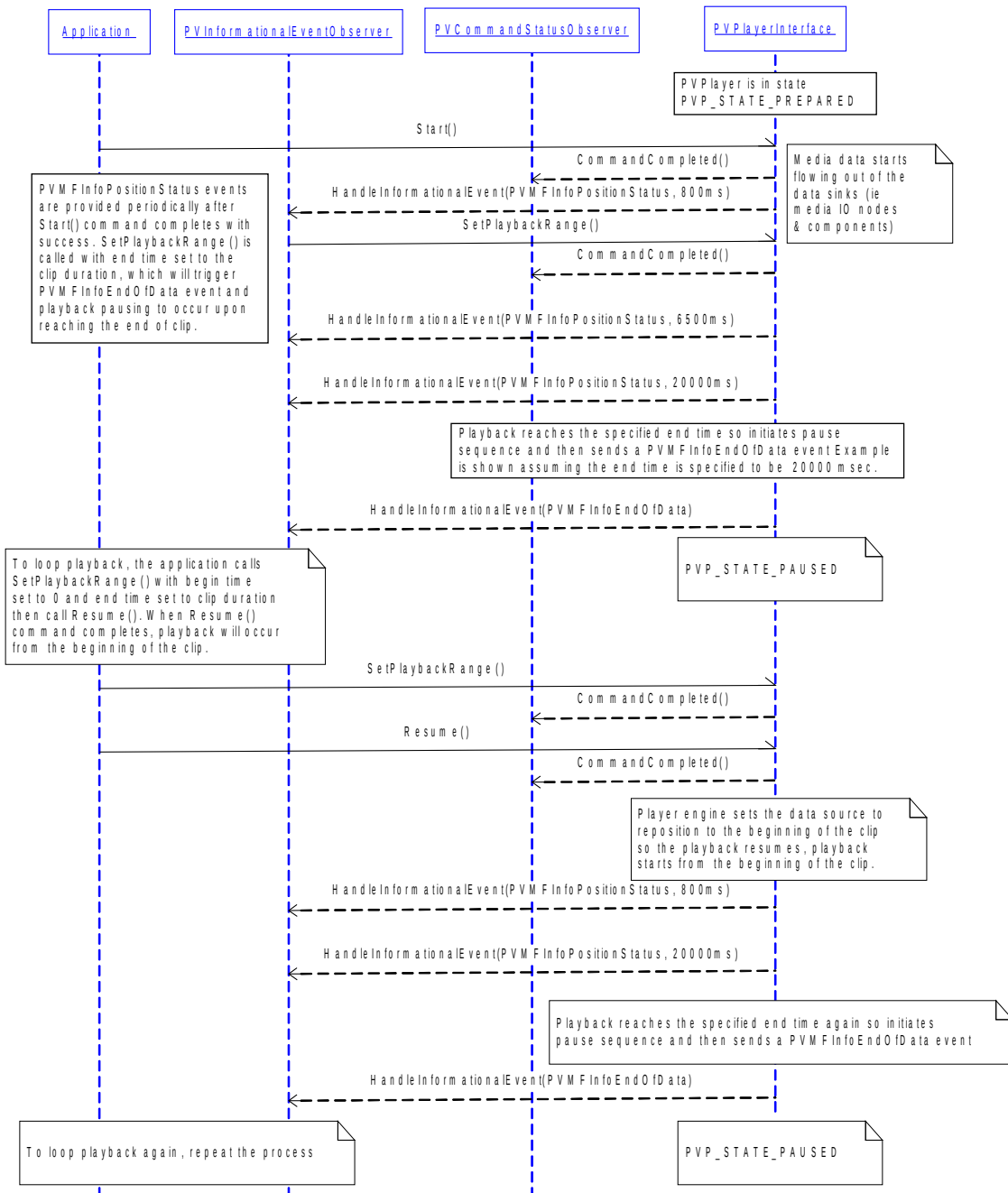
Figure 35: Looped Playback Using SetPlaybackRange
