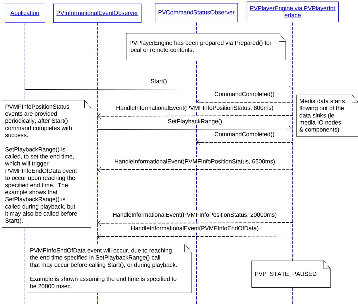
Figure 34: Using SetPlaybackRange and PVMFInfoEndOfData Event
