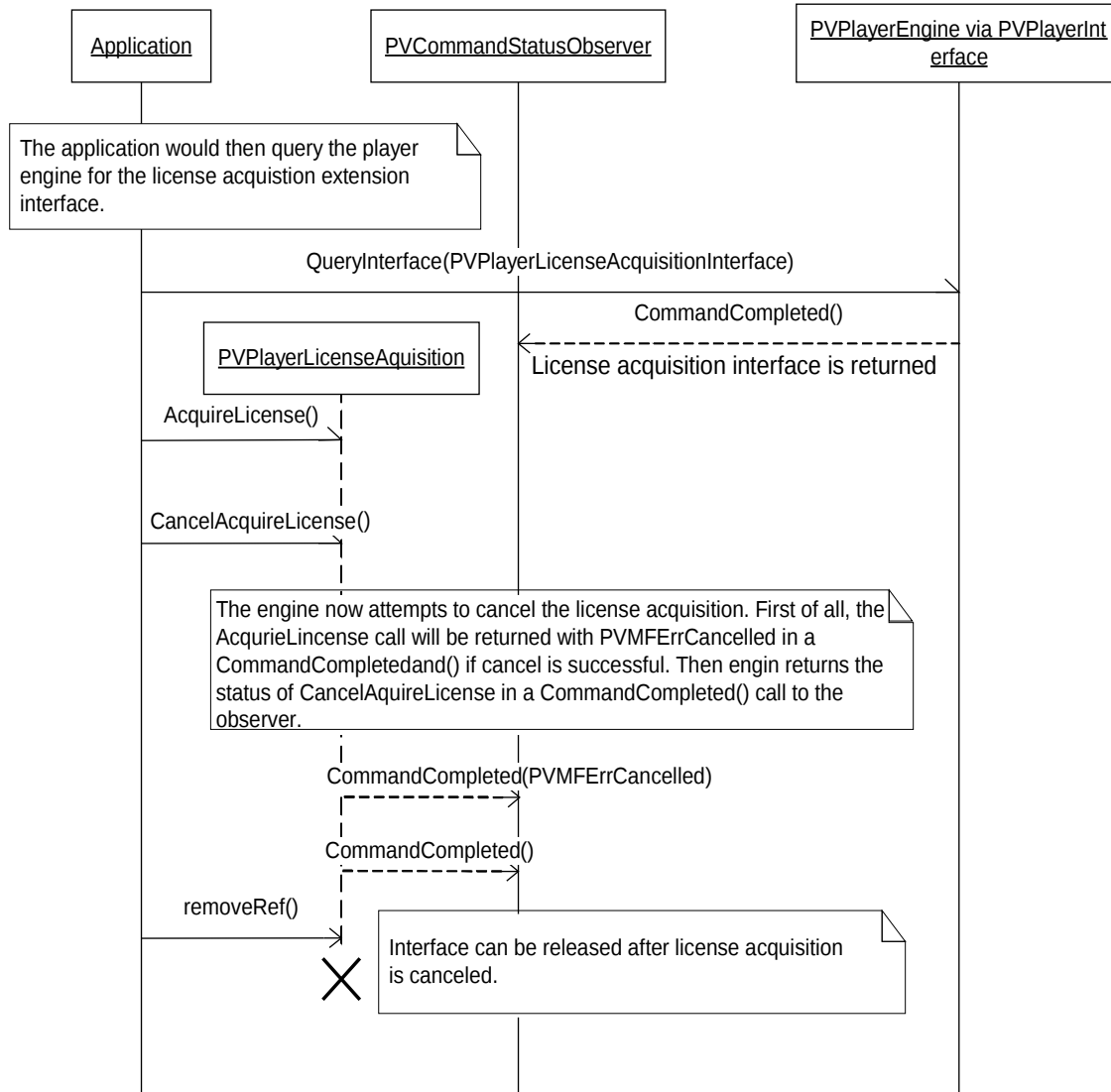
Figure 31: Cancel License Acquisition
