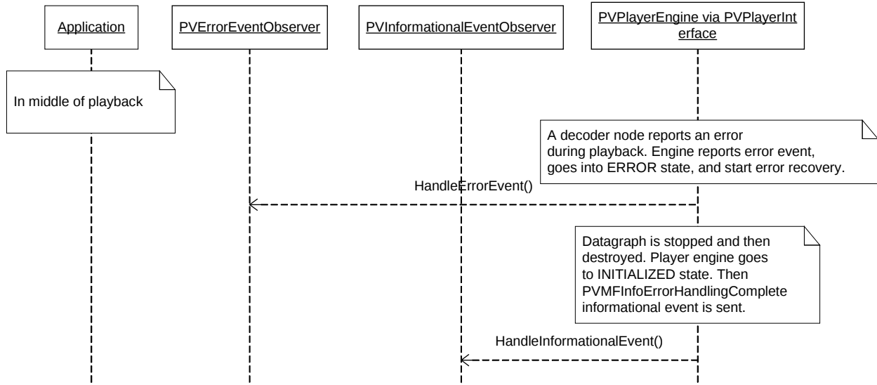
Figure 41: Error Recovery During Playback
