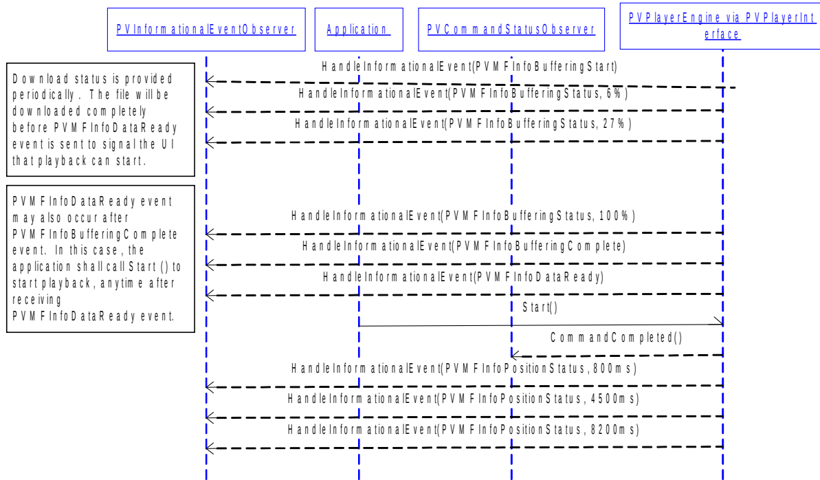
Figure 38: Handling Download Events
