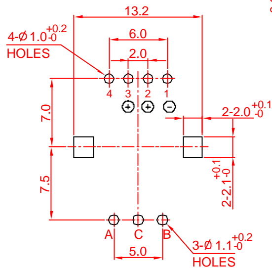
P.W.B MOUNTING DETAIL (TOLERANCE ±0.1) VIEWED FROM MOUNTING SIDE (P.C.B) t=1.5mm
