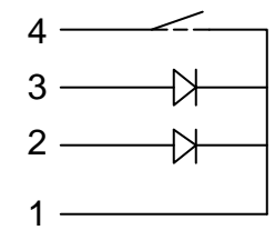
(SW02) CIRCUIT DIAGRAM
