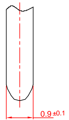
DETAIL OF TERMINAL (5:1)
